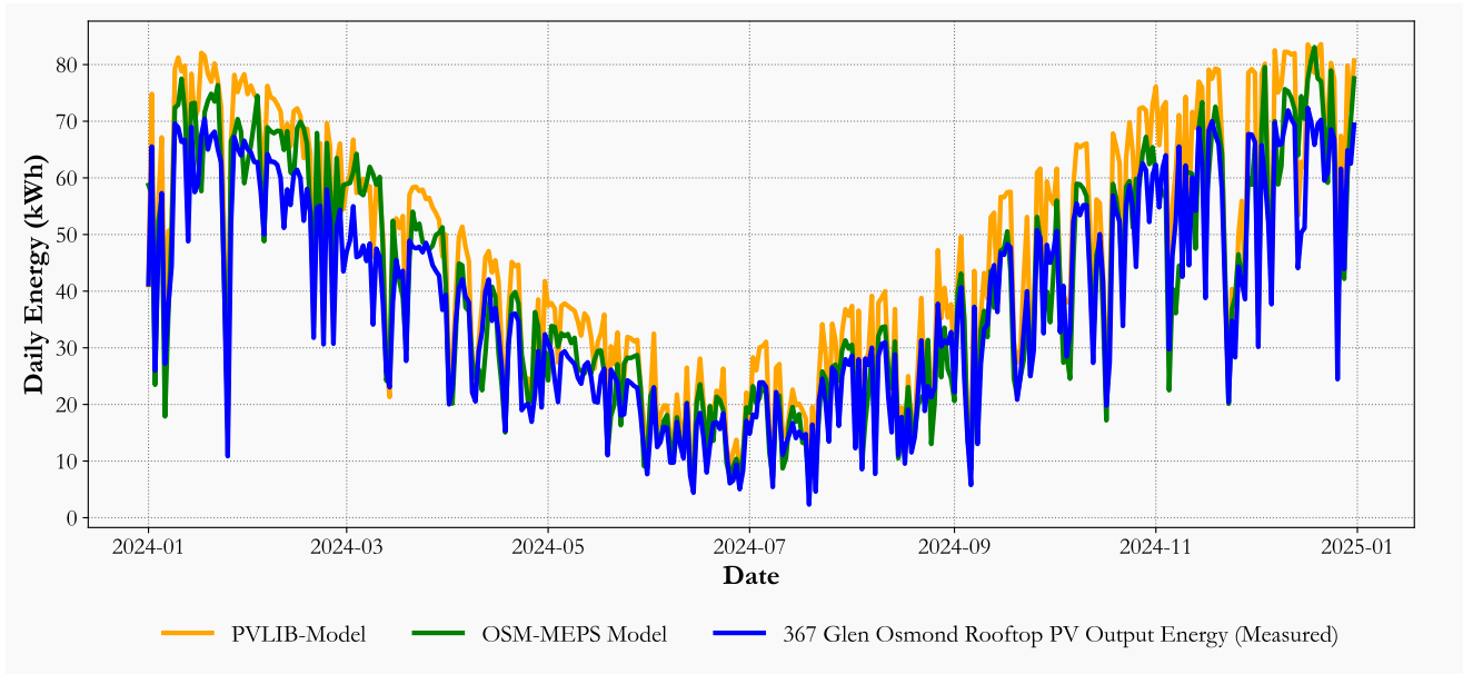
FIGURE 27. Comparison of PVLIB and OSM-MEPS modeled solar PV energy with measured data at 367 Glen Osmond rooftop, Adelaide, Australia.
