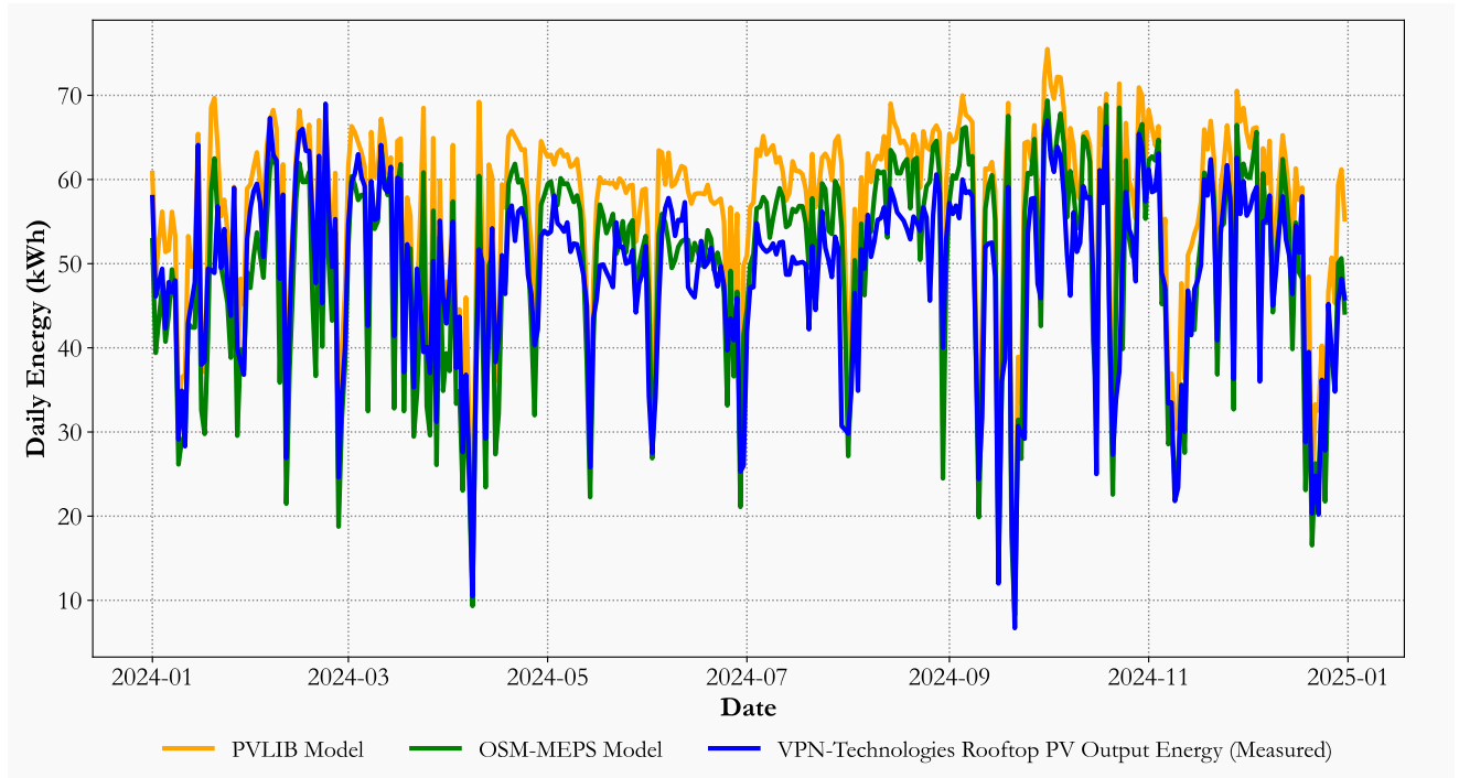
FIGURE 25. Comparison of PVLIB and OSM-MEPS model solar PV energy results with VPN Technologies rooftop PV energy data, Pretoria, South Africa.
