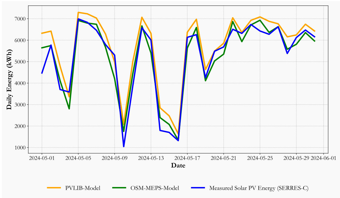
FIGURE 15. Comparison of Serres-C measured energy generation [76] with PVLIB and OSM-MEPS model results for May 2024.
