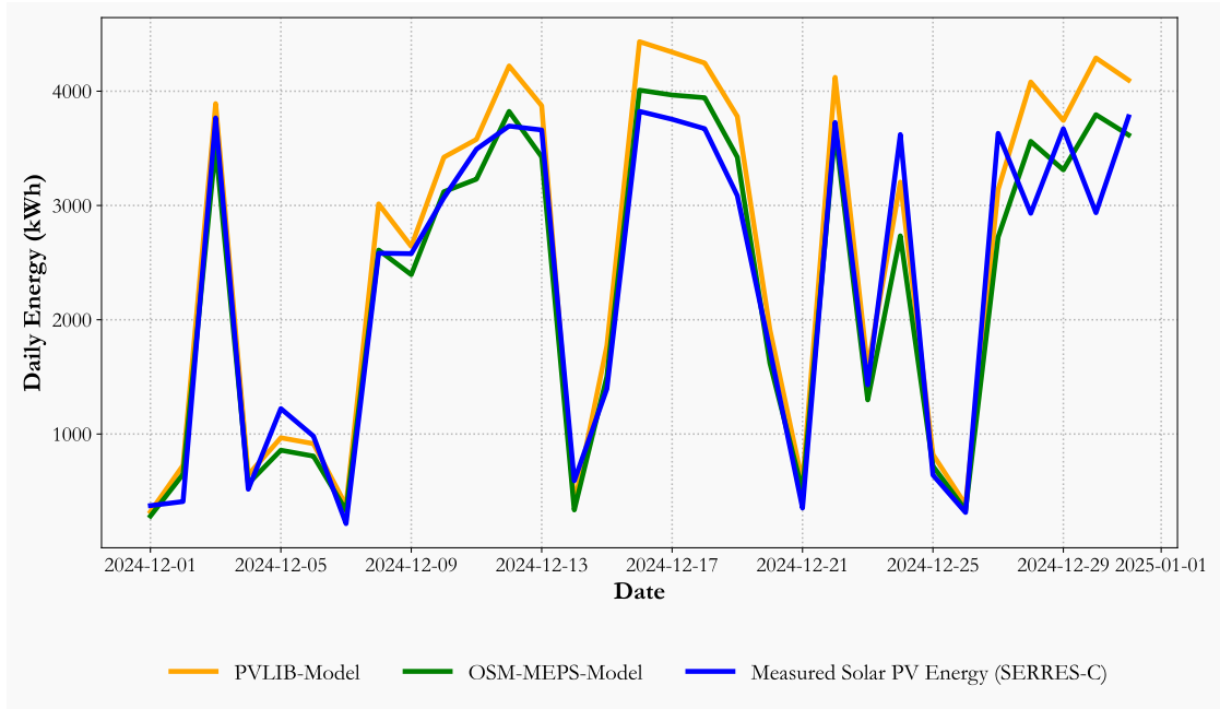
FIGURE 14. Comparison of Serres-C measured energy generation [76] with PVLIB and OSM-MEPS model results for December 2024.
