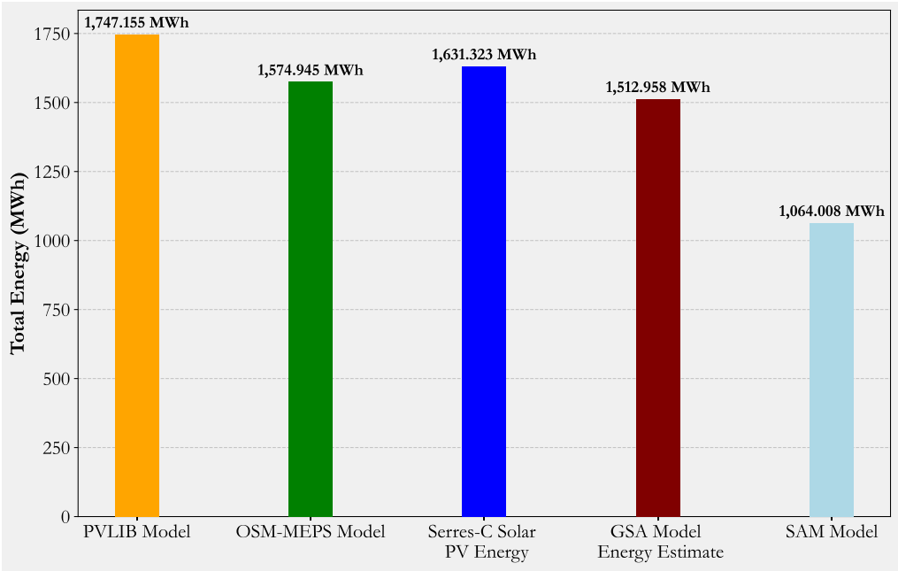
FIGURE 18. Comparison of modeled 2024 solar PV energy yield—using PVLIB, OSM-MEPS, GSA and SAM—with actual measured energy output (MWh) at the Serres-C power plant.
