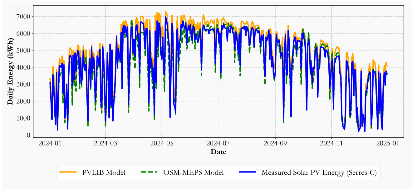
FIGURE 16. Comparison of PVLIB and OSM-MEPS model solar PV energy results with Serres-C PV power plant output, Serres, Greece.
