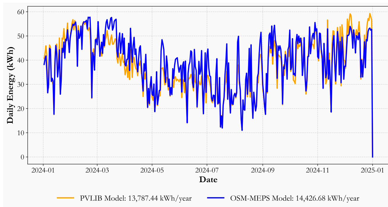
FIGURE 32. Daily energy production for 2024 at Njagu-Mhasibu-Ruiru Estate, Kenya, with a solar panel surface azimuth of 90^\circ and tilt angle of 22.5^\circ .
